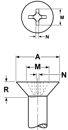
Phillips
