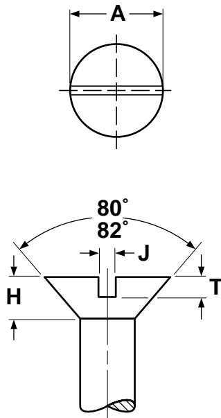
Slotted
