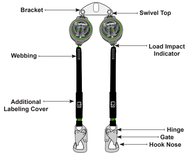
FIGURE 9 - EXAMPLES OF EQUIPMENT DAMAGE
