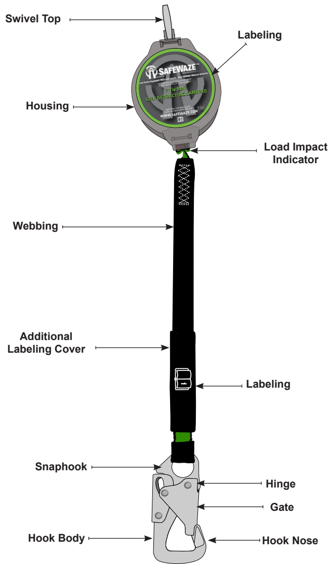
FIGURE 8 - INSPECTION DIAGRAMS
