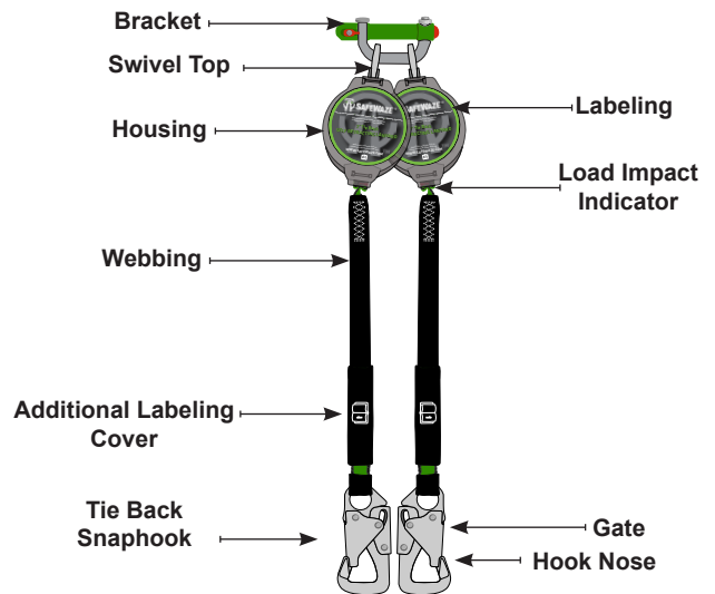
FIGURE 8 - INSPECTION DIAGRAMS
