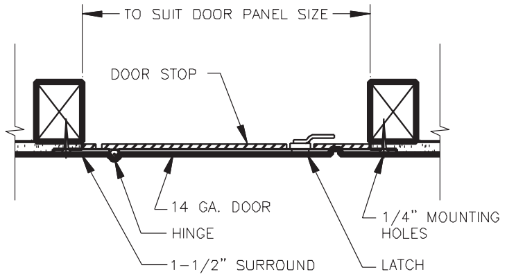
SECTION DETAIL
